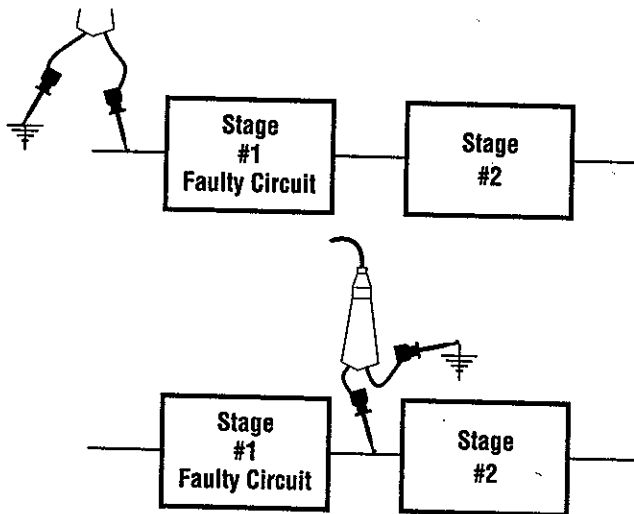
Fig. 47 - Use signal injection to narrow a problem down to a single stage.
