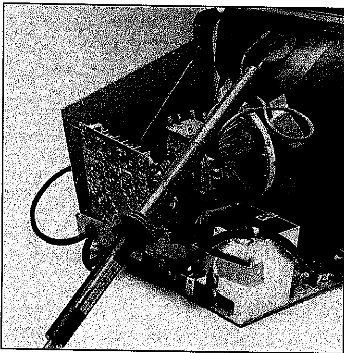
Fig. 63 - Use caution when measuring high voltage with the HP200, 50,000 volt high voltage probe.
