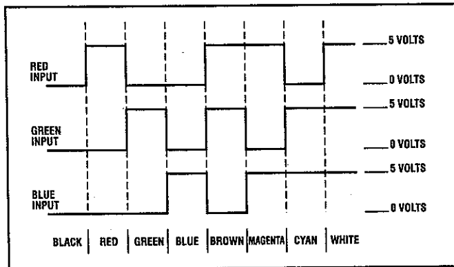
Fig. 37 - The signal input to digital monitors is either a logic low or a logic high.
